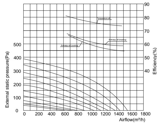
Heat Recovery Ekaffes 130 Performance Chart
