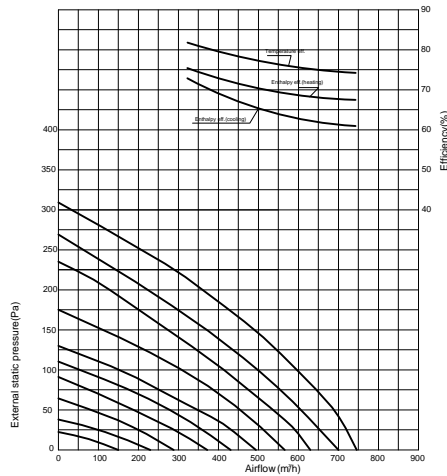
Heat Recovery Ekaffes 065 Performance Chart
