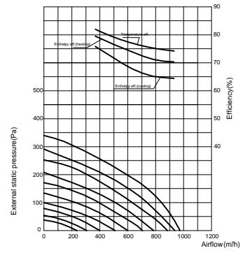
Heat Recovery Ekaffes 080 Performance Chart
