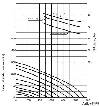
Heat Recovery Ekaffes 100 Performance Chart
