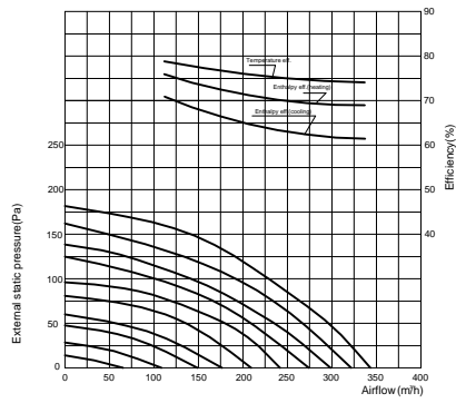
Heat Recovery Ekaffes 025 Performance Chart
