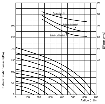
Heat Recovery Ekaffes 050 Performance Chart
