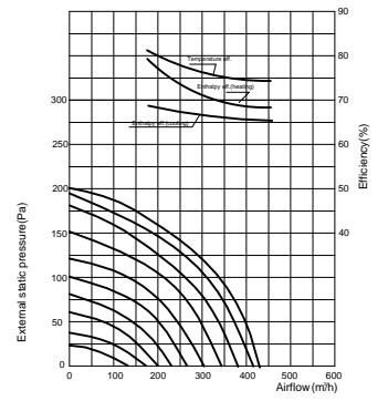
Heat Recovery Ekaffes 035 Performance Chart
