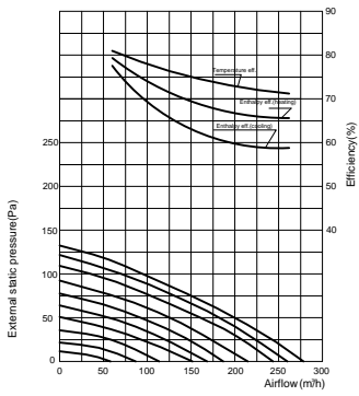
Heat Recovery Ekaffes 015 Performance Chart
